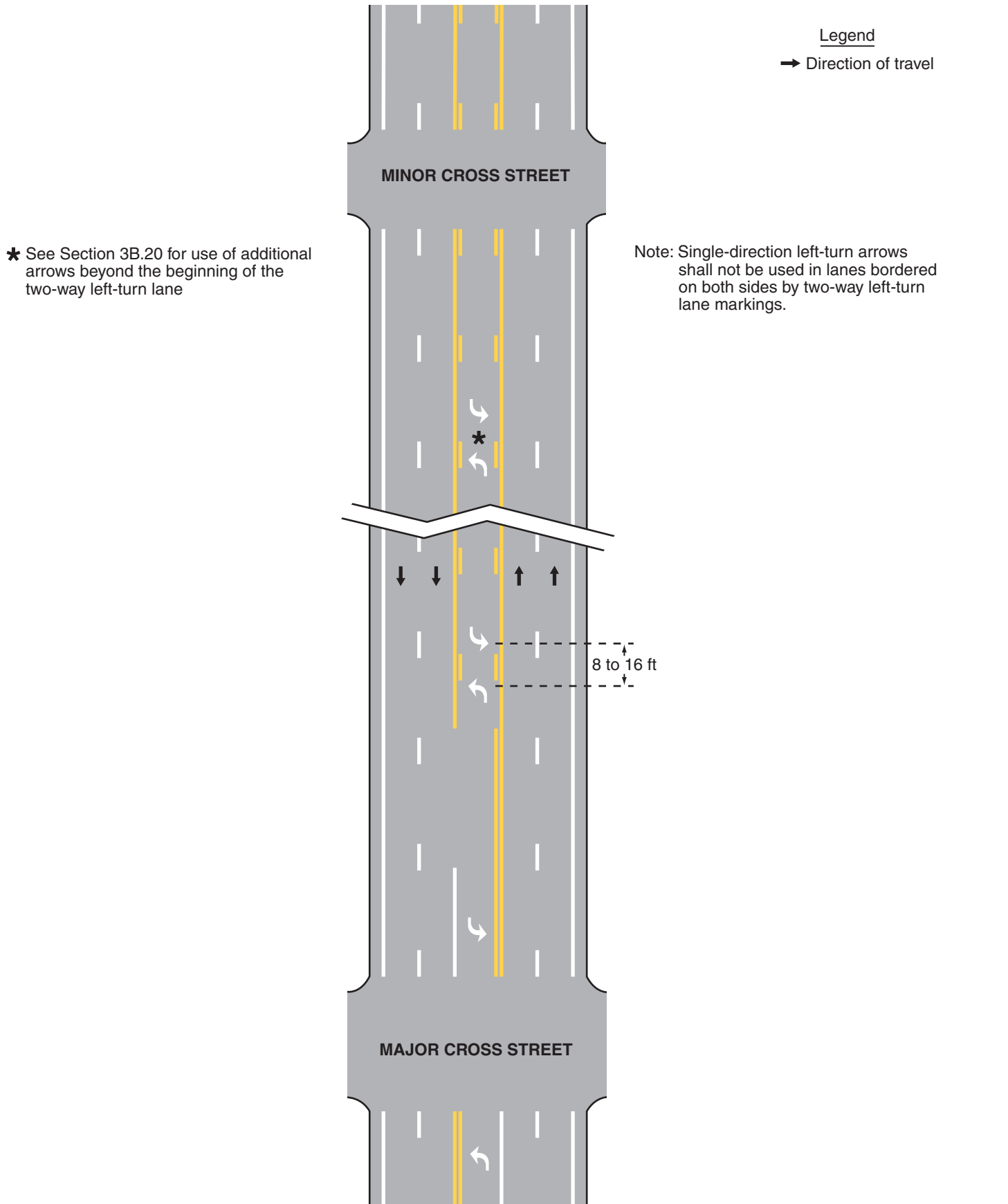
Figure 3B-7. Example of Two-Way Left-Turn Lane Marking Applications
